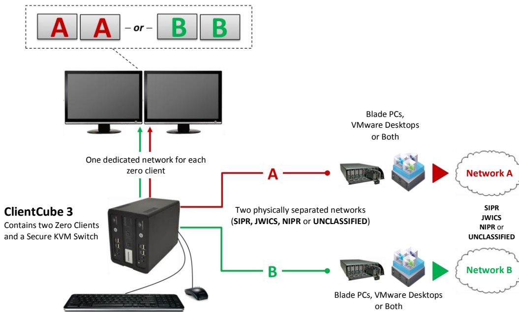
Figure 3. Overview of typical ClientCube 3 deployment
