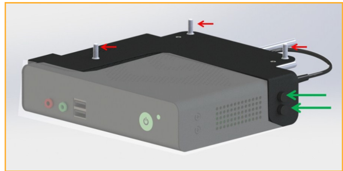
Top side— Under desk mounted bracket
